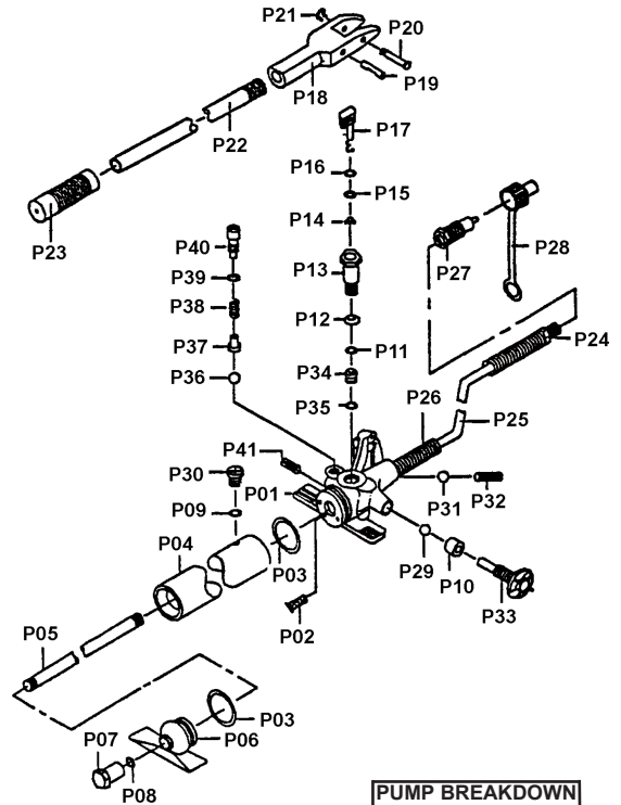
PUMP BREAKDOWN
